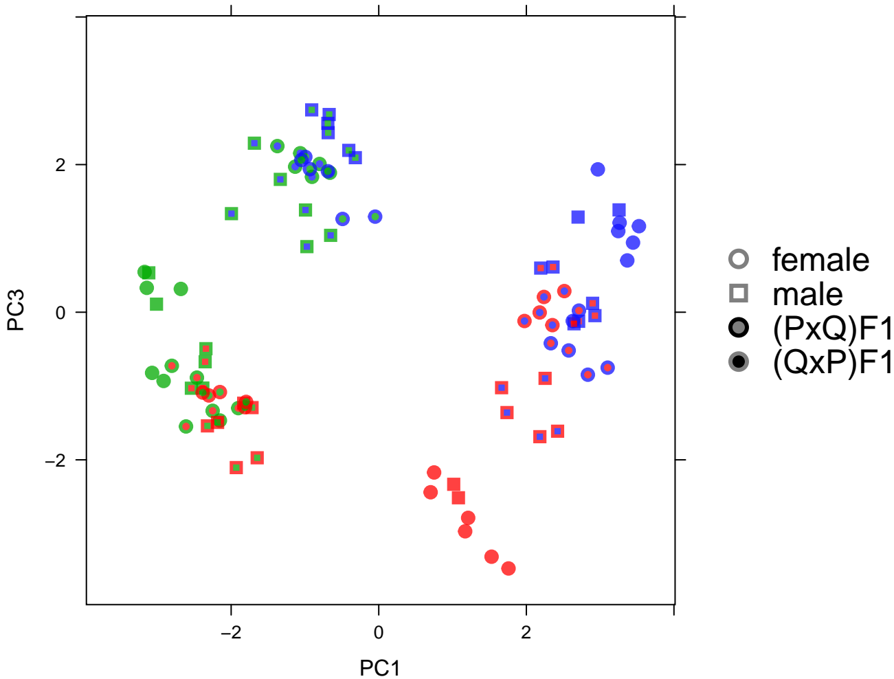
X chromosome total read count (TReC) PC1 vs PC3 (symbol size = 1.0)
