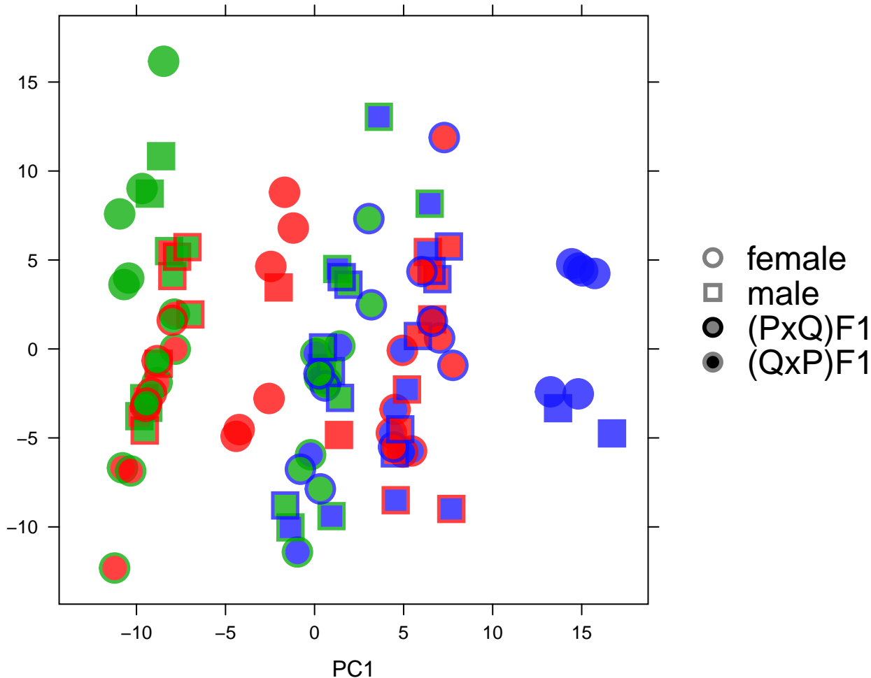
Autosomal total read count (TReC) PC1 vs PC3 (symbol size = 2.5)
