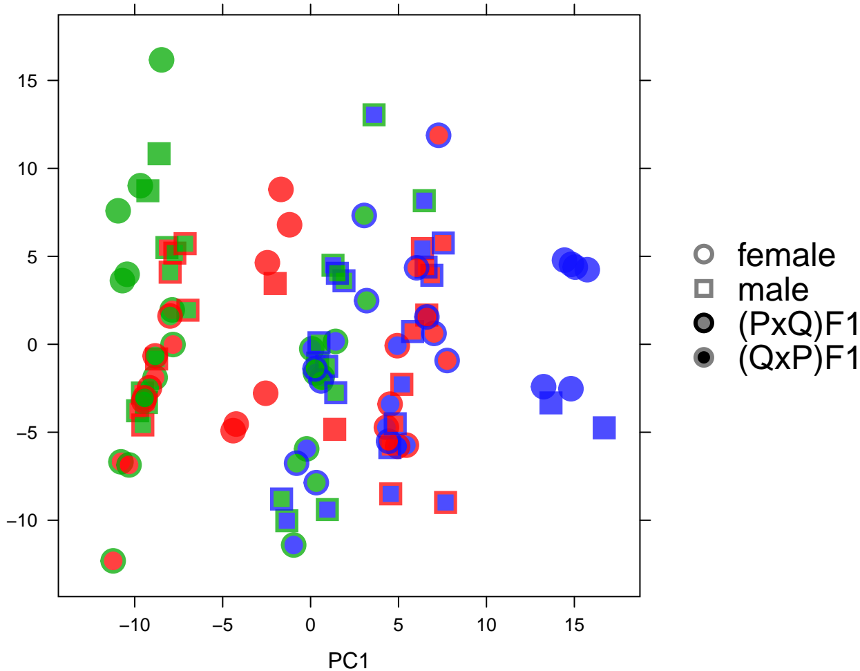
Autosomal total read count (TReC) PC1 vs PC3 (symbol size = 2.0)
