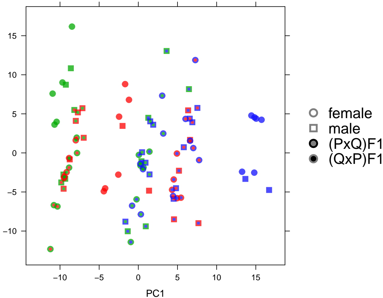
Autosomal total read count (TReC) PC1 vs PC3 (symbol size = 1.0)
