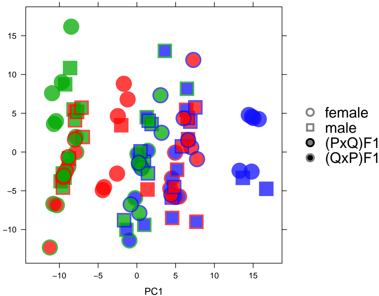
Autosomal total read count (TReC) PC1 vs PC3 (symbol size = 3.0)
