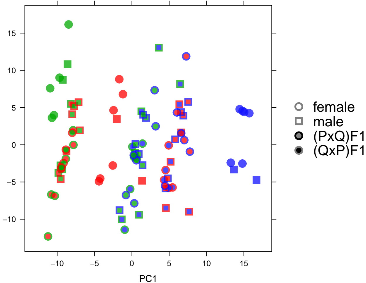
Autosomal total read count (TReC) PC1 vs PC3 (symbol size = 1.5)
