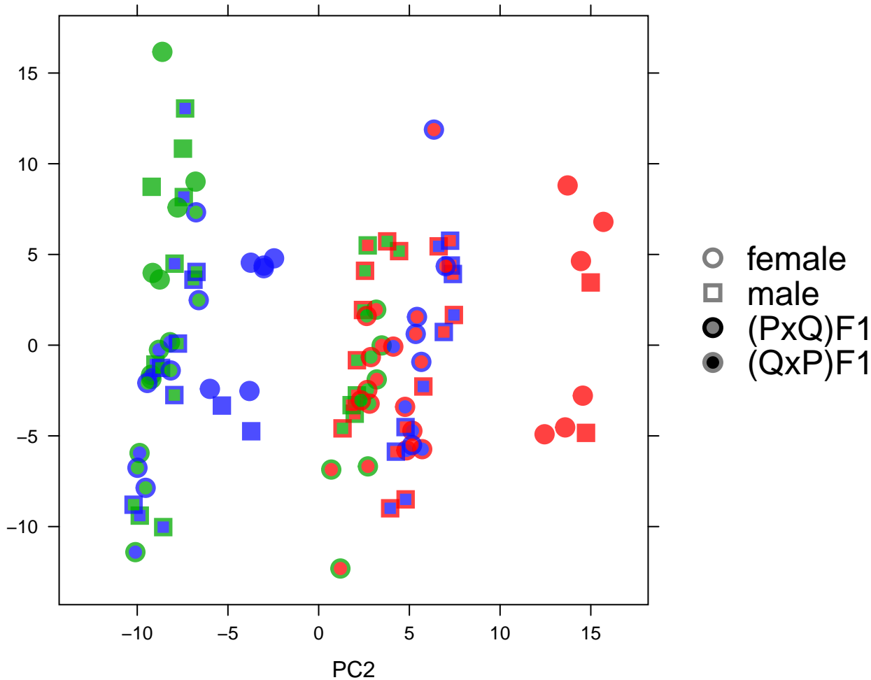
Autosomal total read count (TReC) PC2 vs PC3 (symbol size = 1.5)
