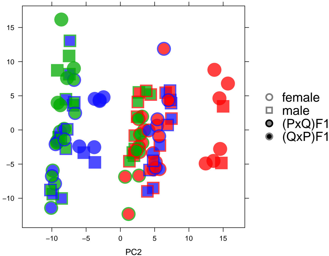
Autosomal total read count (TReC) PC2 vs PC3 (symbol size = 3.0)
