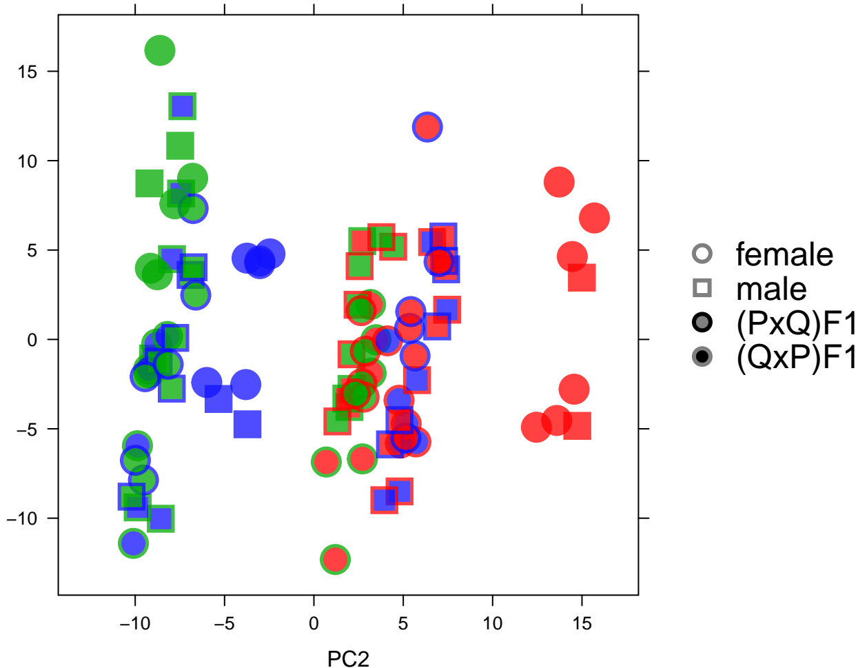
Autosomal total read count (TReC) PC2 vs PC3 (symbol size = 2.5)
