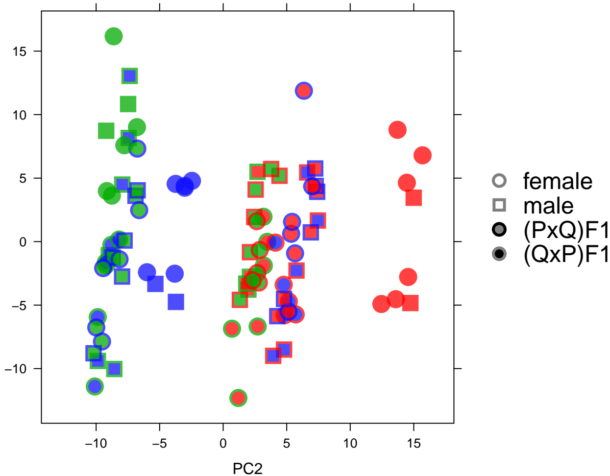
Autosomal total read count (TReC) PC2 vs PC3 (symbol size = 2.0)
