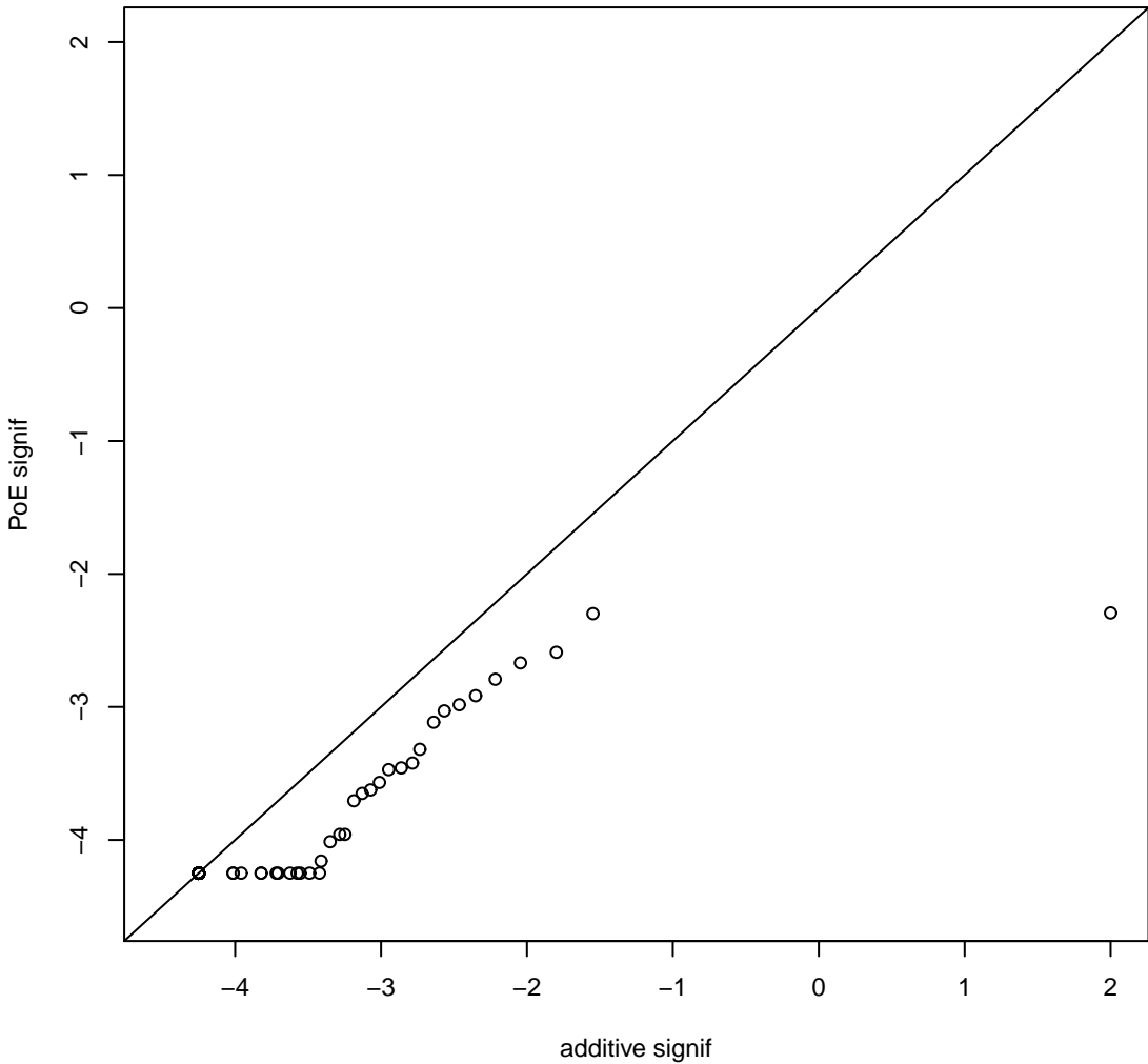
FG, thetas of additive vs PoE
